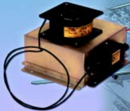
Pedestal Display Box and AFT Avionics Fan EMI Filter / LSWD / Chassis Assembly
